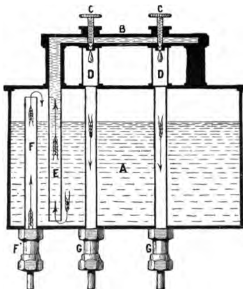
FIG. 385.—Typical Force-feed Lubricator, operating by air or gas pressure, instead of a pump. The parts are: A, oil reservoir; B, distributing pipe; C, C, valve screws for regulating flow of oil to parts, through leaders. D and D'; E, standpipe through which oil is forced by air pressure; F, standpipe admitting gas from crank case of engine; F', union for pipe from crank case; G, G, unions for pipes to various parts of the machinery.
